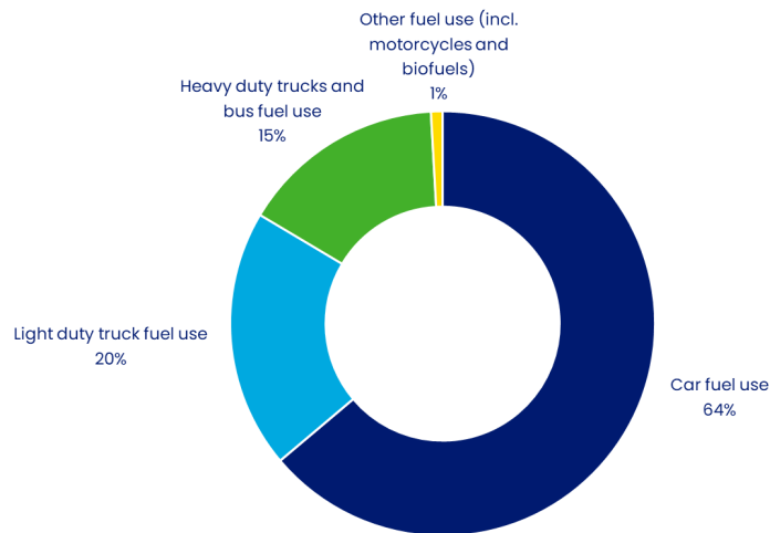
Figure 1: Road transport GHG emissions in Wales in 2023
