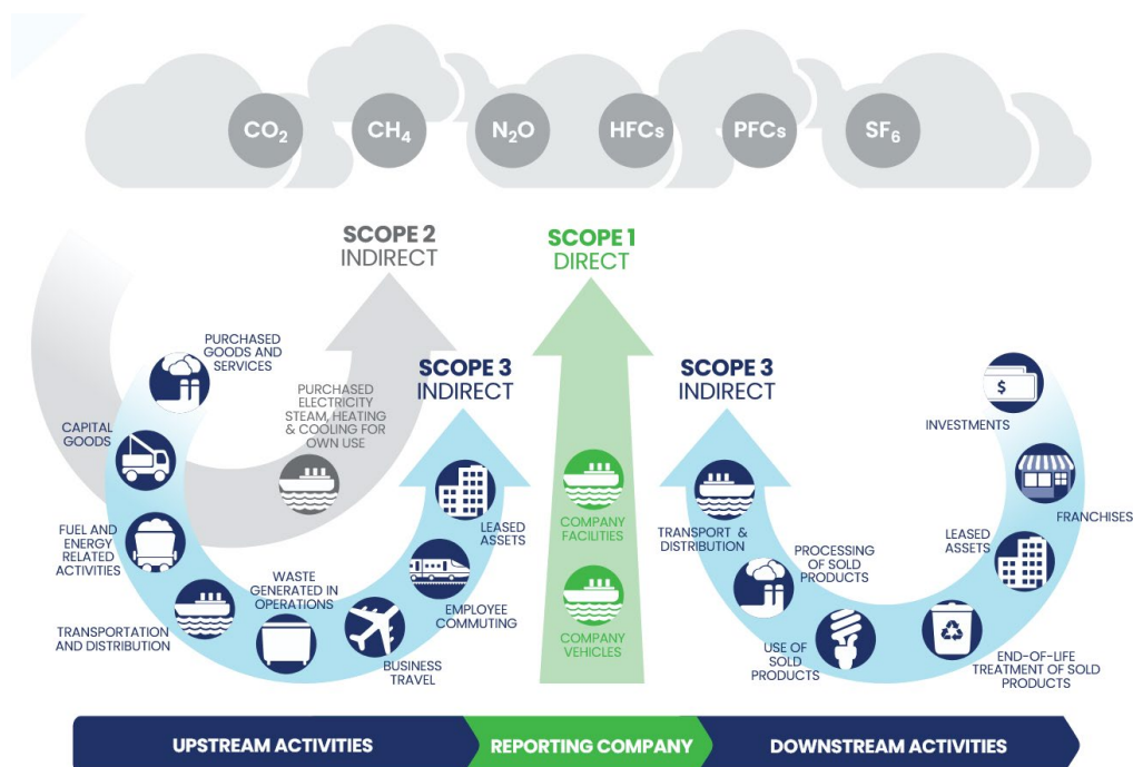
Figure 2: Corporate GHG emission measurement and reporting sources.
